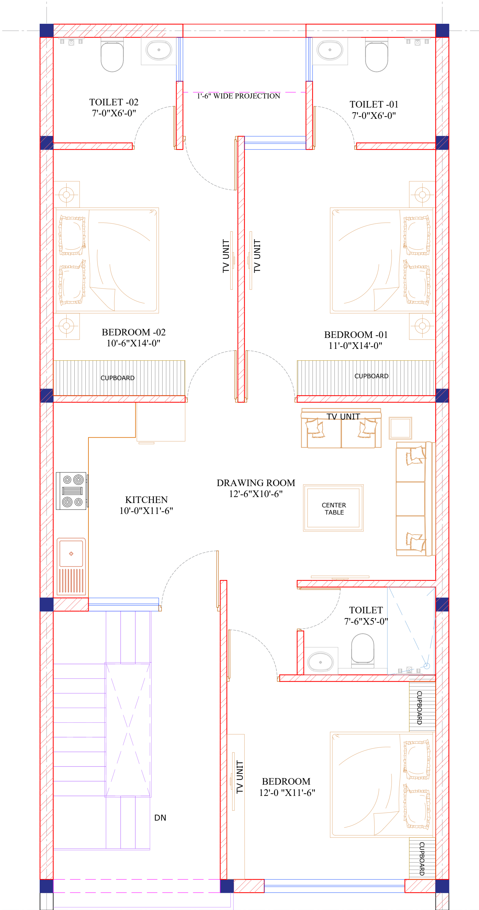
GROUND FLOOR PLAN 22'-6" x 50'-0"
