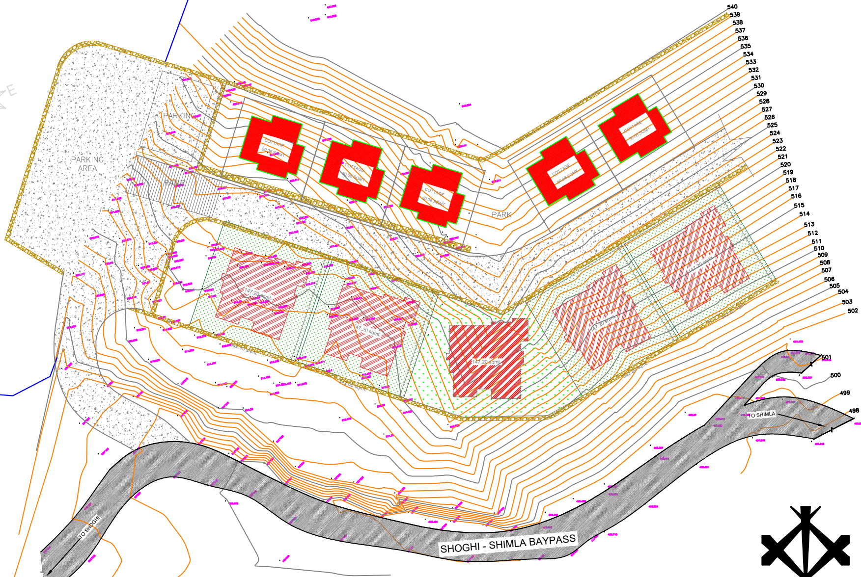
SITE AND CONTOUR PLAN
