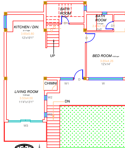
GROUND FLOOR PLAN AREA 90.45 SQMT
